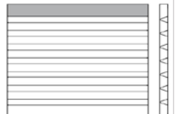
SQG-PBG GRID 22 8 Division/Div. Size of Each Division 1.97"x20.16" (50x512 mm)
